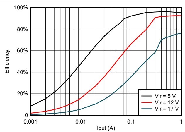
Figure 6-8. TPSM861253 Efficiency
