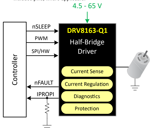
Simplified Schematic
