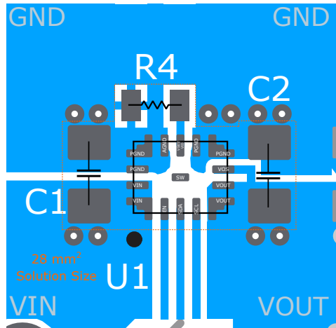
Figure 9-28. Layout Example
