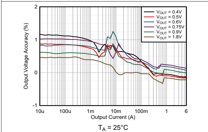
Figure 9-12. Load Regulation V_{IN} = 2.8V and PSM
