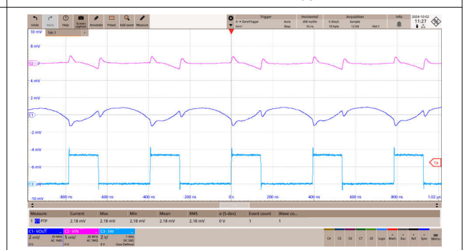
Figure 9-17. PSM Operation I_{OUT} = 0.1A
