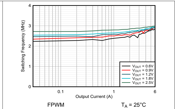
Figure 9-15. Switching Frequency V_{IN} = 3.3V
