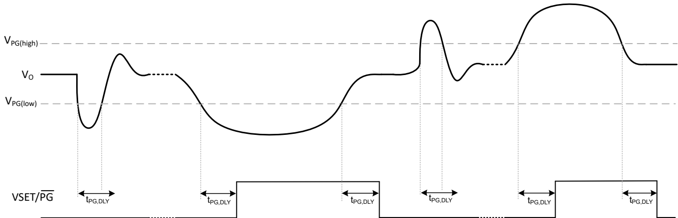
Figure 7-3. VSET/P \overline{\text{G}} Transient and Delay Behavior
