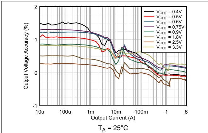
Figure 9-8. Load Regulation V_{IN} = 5.0V and PSM
