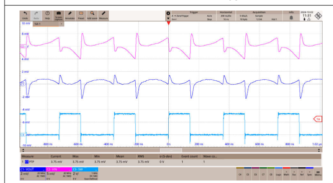
Figure 9-16. FPWM Operation I_{OUT} = 3A
