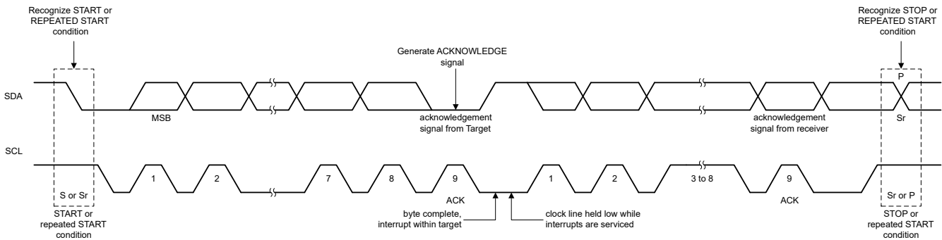
Figure 7-7. Bus Protocol
