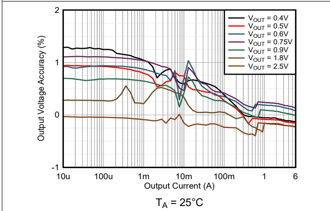
Figure 9-10. Load Regulation V_{IN} = 3.3V and PSM
