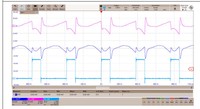
Figure 9-14. Switching Frequency V_{IN} = 5.0V
