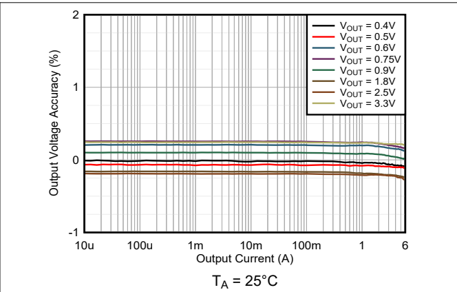
Figure 9-9. Load Regulation V_{IN} = 5.0V and FPWM
