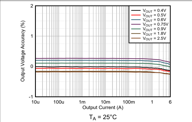
Figure 9-11. Load Regulation V_{IN} = 3.3V and FPWM
