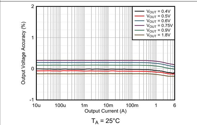
Figure 9-13. Load Regulation V_{IN} = 2.8V and FPWM
