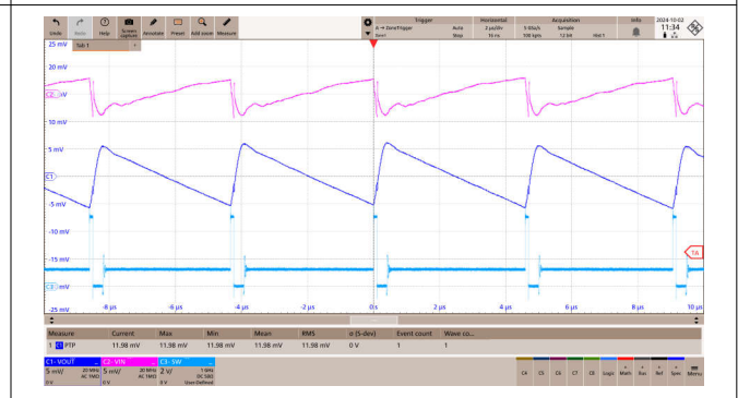
Figure 9-15. Switching Frequency V_{IN} = 3.3V
