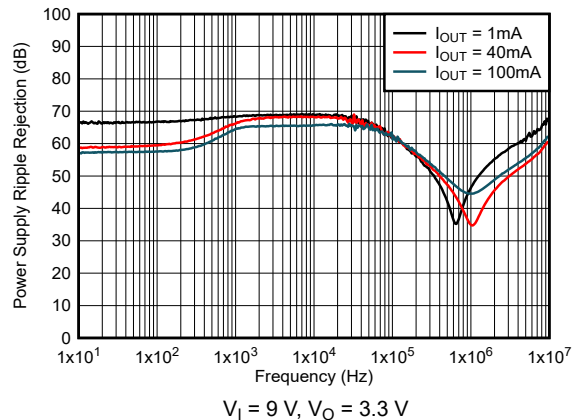
Figure 6-22. PSRR vs Frequency and I_O for New Chip V_I = 9\text{ V} , V_O = 3.3\text{ V}
