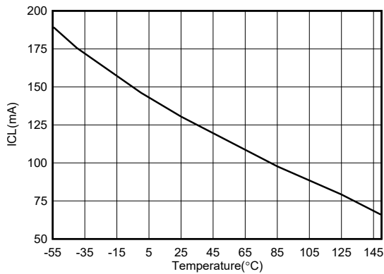
Figure 6-19. I_{CL} vs Temperature for New Chip V_O = 90\% of V_O (typ)
