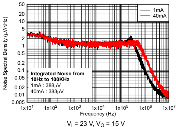
Figure 6-21. Noise Spectral Density vs Frequency and I_O for New Chip V_I = 23\text{ V} , V_O = 15\text{ V}
