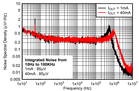
Figure 6-20. Noise Spectral Density vs Frequency and I_O for New Chip V_I = 9\text{ V} , V_O = 3.3\text{ V}
