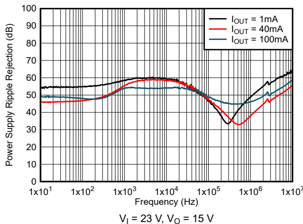
Figure 6-23. PSRR vs Frequency and I_O for New Chip V_I = 23\text{ V} , V_O = 15\text{ V}
