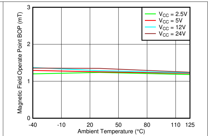
Figure 6-2. B OP_Z Threshold vs Temperature
