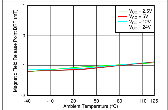
Figure 6-4. B RP_Z Threshold vs Temperature
