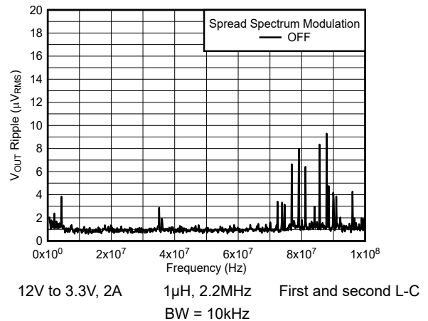
Figure 5-12. V_{OUT} Ripple FFT After the Second L-C Filter
