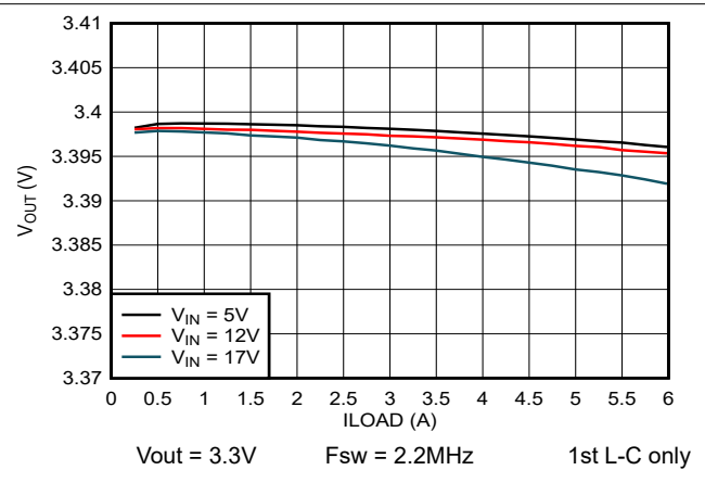
Figure 7-3. Output Voltage vs Load Current
