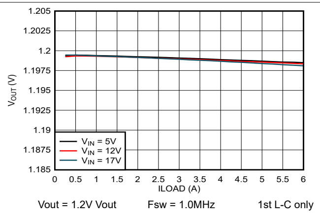
Figure 7-7. Output Voltage vs Load Current
