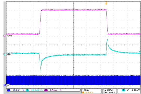
Figure 7-17. Load Transient
