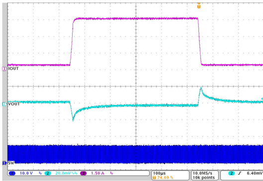
Figure 7-16. Load Transient
