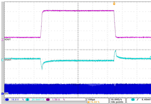
Figure 7-14. Load Transient
