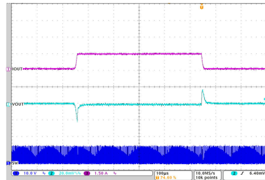
30mA to 1.5A to 30mA 12V to 1.2V 1μH, 1MHz After 2nd L-C
