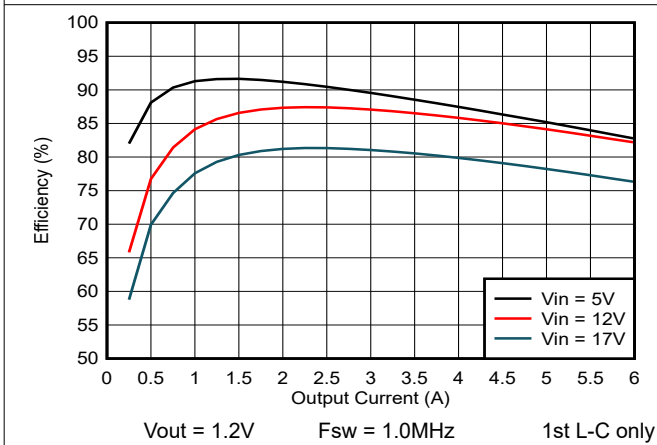
Figure 7-6. Efficiency vs Load Current
