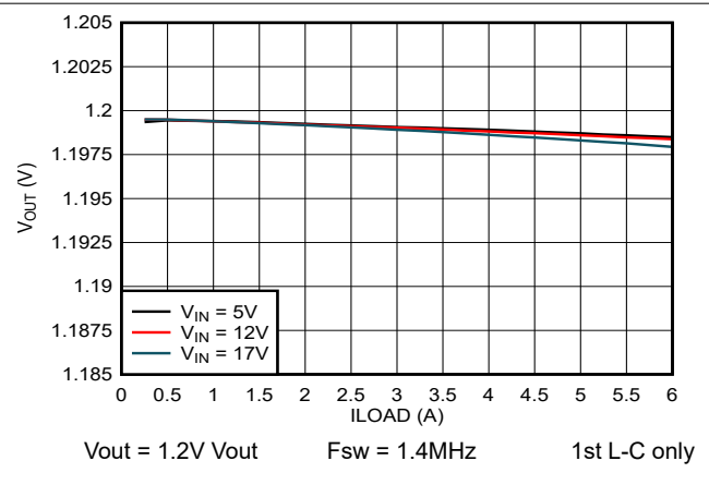
Figure 7-5. Output Voltage vs Load Current
