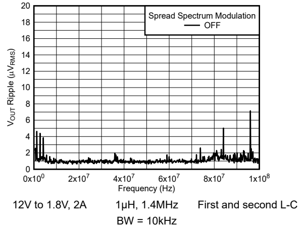
Figure 5-8. V_{OUT} Ripple FFT After the Second L-C Filter
