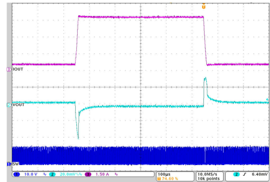
Figure 7-15. Load Transient
