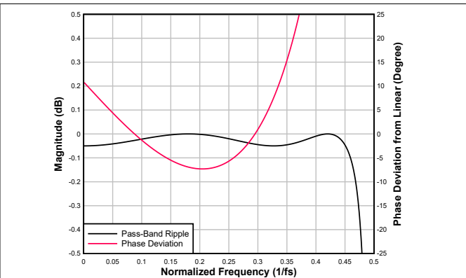
Figure 6-100. Ultra-Low-Latency interpolation Filter Pass-Band Ripple and Phase Deviation
