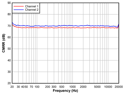
DC-coupled differential line input
