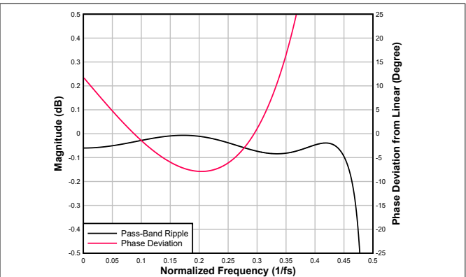
Figure 6-98. Ultra-Low-Latency interpolation Filter Pass-Band Ripple and Phase Deviation
