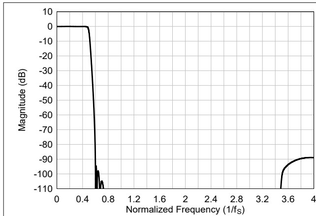
Figure 6-97. Ultra-Low-Latency interpolation Filter Magnitude Response
