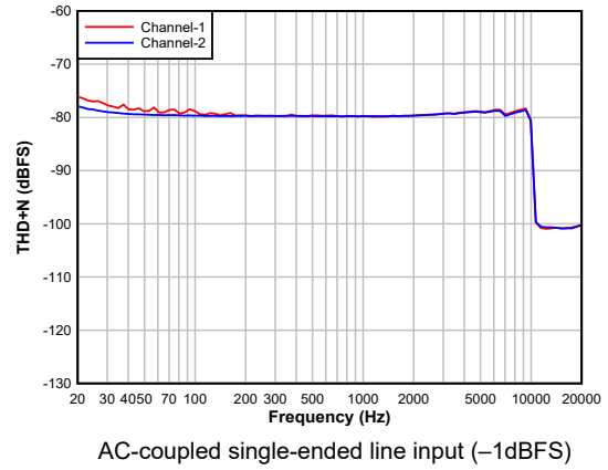
Figure 5-10. ADC THD+N vs Frequency
