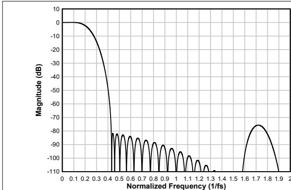
Figure 6-40. Linear-phase Decimation Filter Magnitude Response
