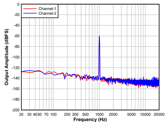
Differential line output
