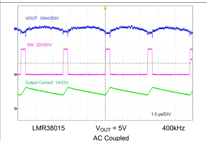
Figure 8-6. Full Load Switching
