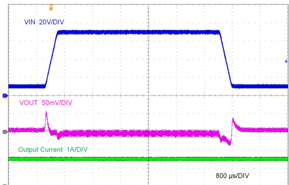
LMR38015 V_{OUT} = 5V 400kHz (AC Coupled)
