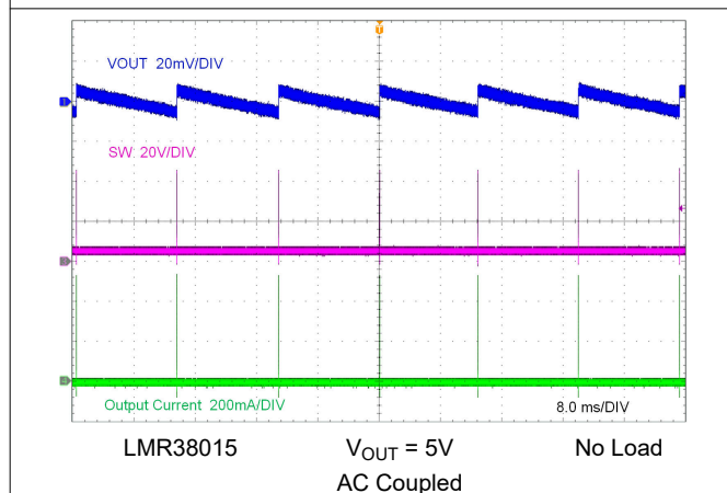
Figure 8-5. PFM Switching
