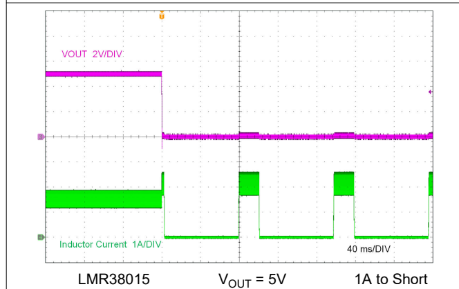
Figure 8-7. Short Circuit Applied
