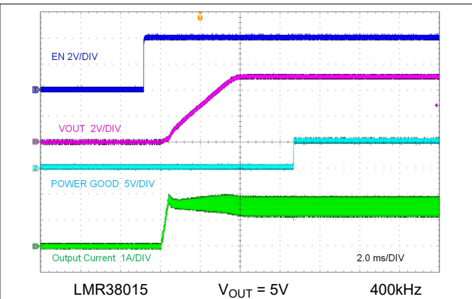
Figure 8-4. Start-Up by EN
