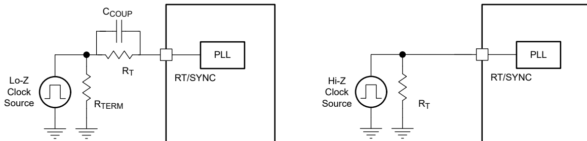
Figure 7-4. Synchronizing to an External Clock
