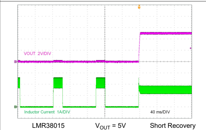
Figure 8-8. Short-Circuit Recovery
