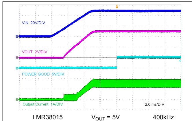
Figure 8-3. Start-Up by VIN
