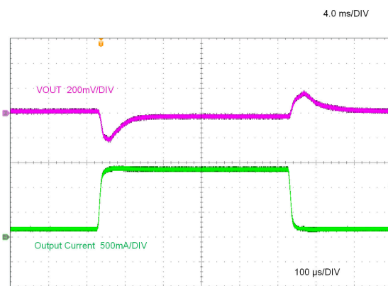
LMR38015 V_{OUT} = 5V 400kHz (AC Coupled)
