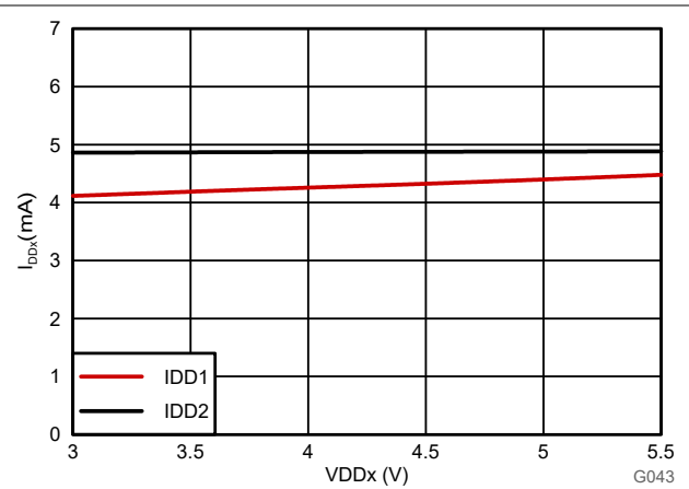
Figure 6-12. Supply Current vs Supply Voltage
