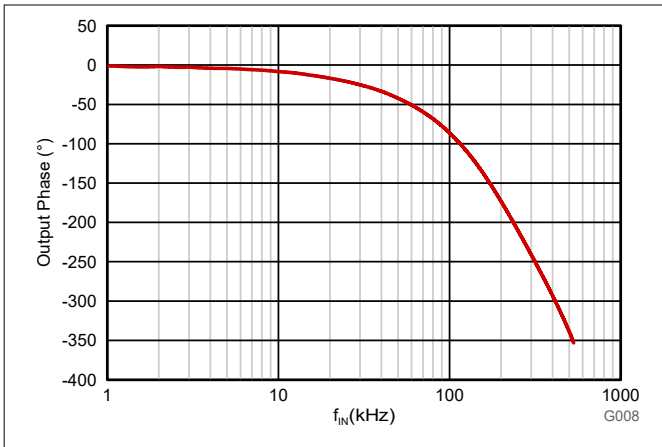
Figure 6-11. Output Phase vs Input Frequency
