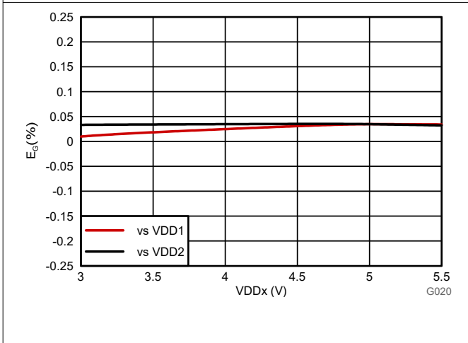
Figure 6-7. Gain Error vs Supply Voltage
