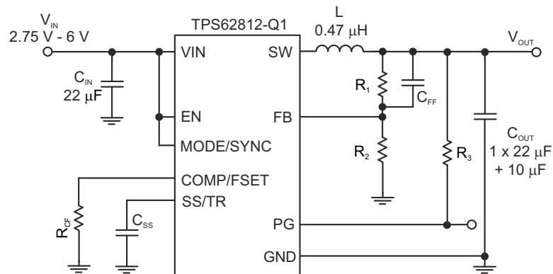
Figure 7-2. Measurement Setup for TPS62812-Q1 and TPS62811-Q1
