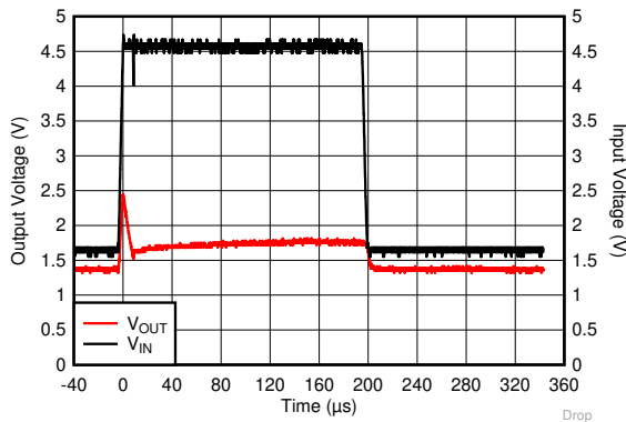
V_{OUT} = 1.8\text{ V} , I_{OUT} = 100\text{ mA} , C_{OUT} = 1\text{ }\mu\text{F} , slew rate = 1\text{ V}/\mu\text{s}
