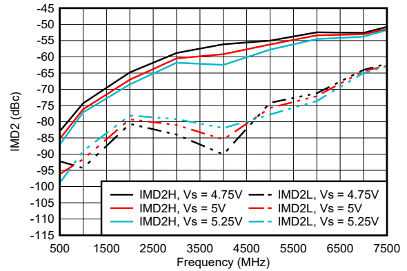
P_O = -5\text{dBm/tone} , 2MHz tone spacing Figure 6-28. IMD2 Across Supply Voltage
