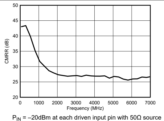
Figure 6-90. Common-Mode Rejection Ratio (CMRR)
