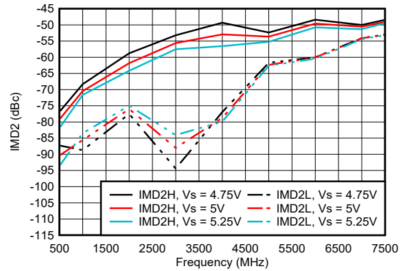
P_O = 1\text{dBm/tone} , 2MHz tone spacing Figure 6-26. IMD2 Across Supply Voltage
