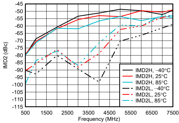
P_O = 1\text{dBm/tone} , 2MHz tone spacing Figure 6-25. IMD2 Across Temperature
