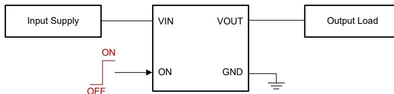
TPS22991I Typical Application
