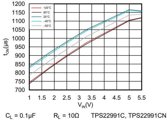
Figure 6-7. Turn ON Time vs Input Voltage
