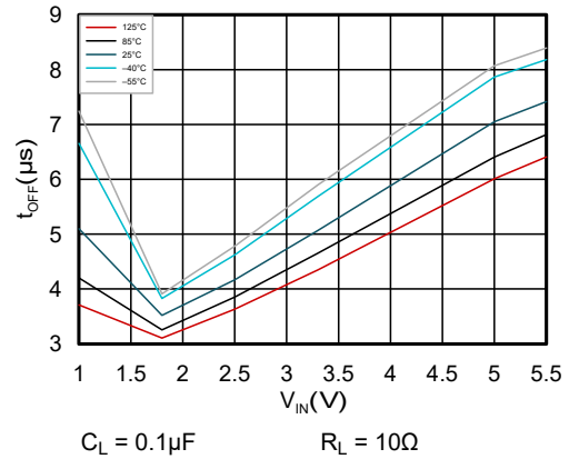
Figure 6-8. Turn OFF Time vs Input Voltage
