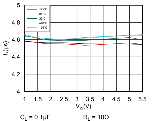
Figure 6-11. Fall Time vs Input Voltage
