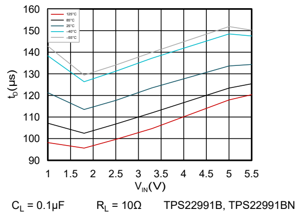
Figure 6-12. Delay Time vs Input Voltage
