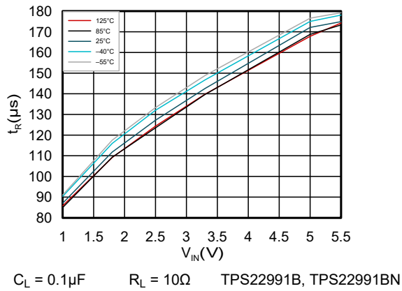
Figure 6-9. Rise Time vs Input Voltage
