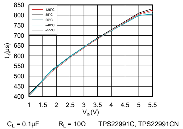
Figure 6-10. Rise Time vs Input Voltage
