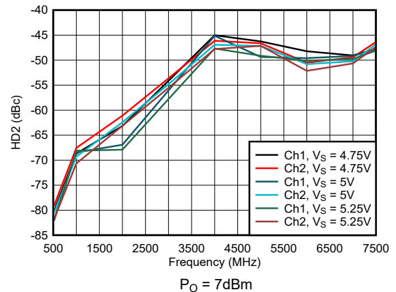
Figure 6-34. HD2 Across Supply Voltage
