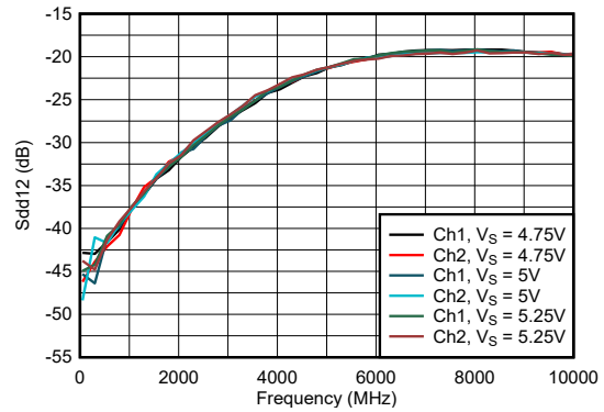
P_{\text{IN}} = -20\text{dBm} with 50\Omega source at all excited ports, nonexcited ports are terminated with 50\Omega
