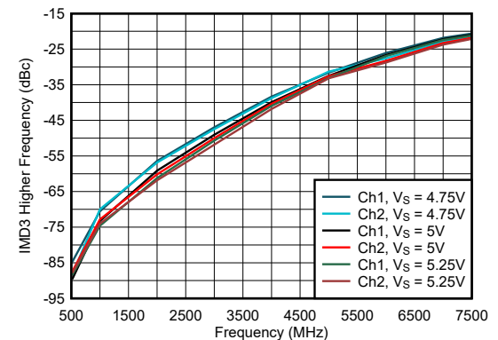
At (2f_2 - f_1) frequency where f_1 < f_2 , P_O = 1\text{dBm/tone} , 2MHz tone spacing
