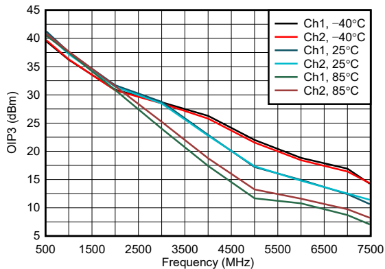
P_O = 1\text{dBm}/\text{tone} , 2MHz tone spacing
