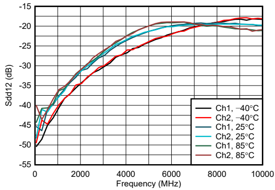
P_{\text{IN}} = -20\text{dBm} with 50\Omega source at all excited ports, nonexcited ports are terminated with 50\Omega
