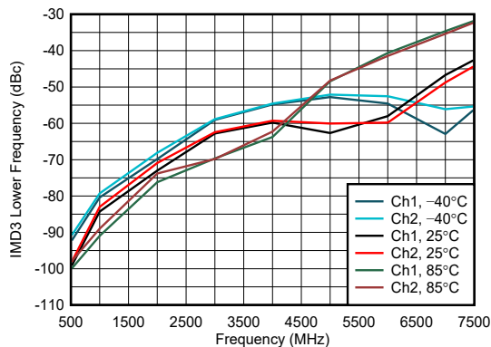
At (2f_1 - f_2) frequency where f_1 < f_2 , P_O = -5\text{dBm/tone} , 2MHz tone spacing
