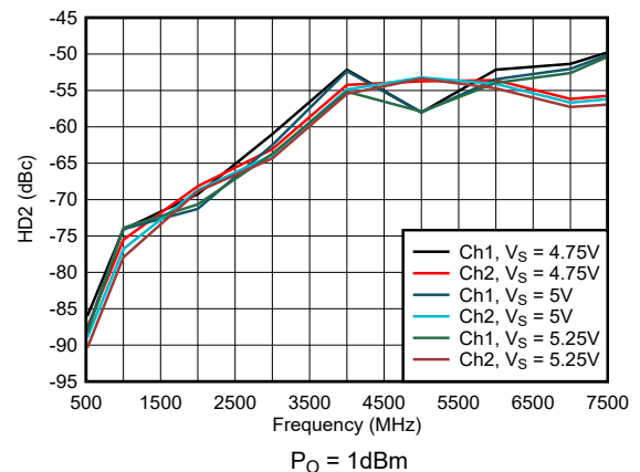
Figure 6-36. HD2 Across Supply Voltage
