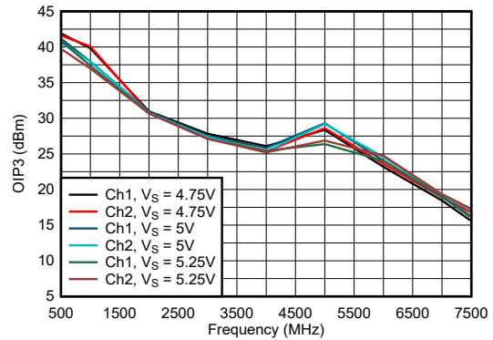
P_O = -5\text{dBm}/\text{tone} , 2MHz tone spacing
