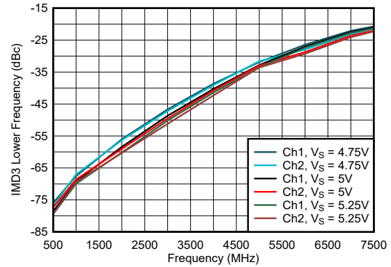
At (2f_1 - f_2) frequency where f_1 < f_2 , P_O = 1\text{dBm/tone} , 2MHz tone spacing
