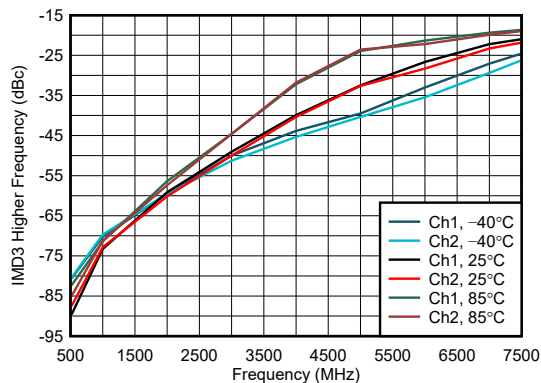
At (2f_2 - f_1) frequency where f_1 < f_2 , P_O = 1\text{dBm/tone} , 2MHz tone spacing
