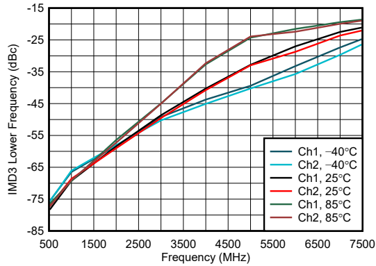
At (2f_1 - f_2) frequency where f_1 < f_2 , P_O = 1\text{dBm/tone} , 2MHz tone spacing
