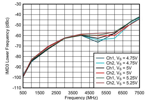
At (2f_1 - f_2) frequency where f_1 < f_2 , P_O = -5\text{dBm/tone} , 2MHz tone spacing
