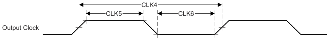
Figure 6-12. Clock Switching Characteristics
