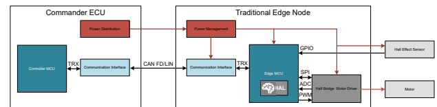
Figure 3. Block diagram of a remote-controlled edge node with communication to a commander ECU.
