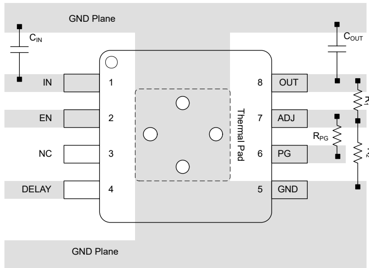
Figure 7-5. Example Layout for TPS7E66-Q1 DGN Package
