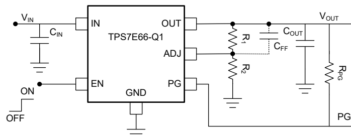
Figure 7-4. Typical Application Circuit (Adjustable-Voltage Version)
