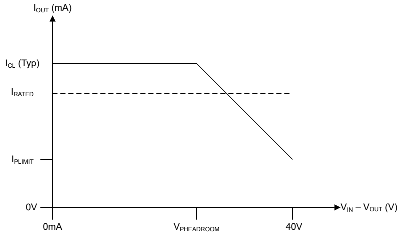
Figure 6-5. Power Limiting
