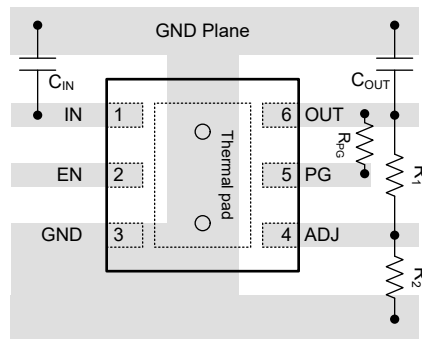
Figure 7-6. Example Layout for TPS7E66-Q1 DRV Package
