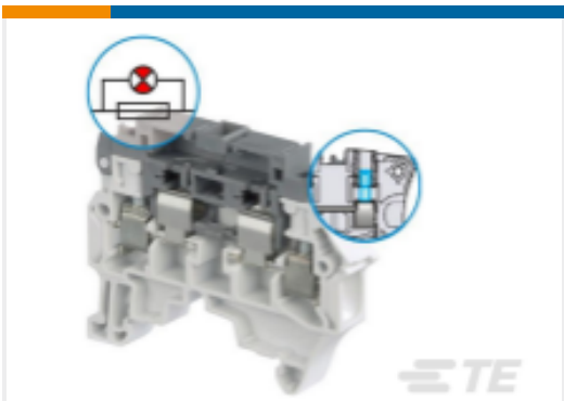
TE Part #1SNK508415R0000 ZS4-SF1-R4
