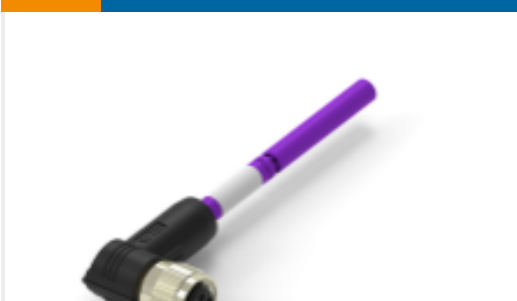
TE Part #TAB62335501-020 Fieldbus,PROFIBUS M12B 2p PUR Drag Chain
