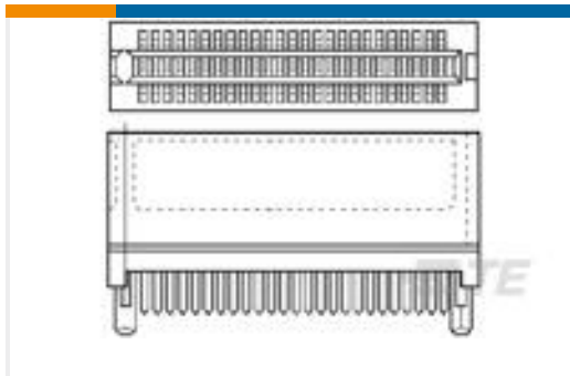
TE Part #5650719-1 STANDARD EDGE .050 SERIES 25 DUAL ASSY
