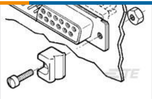
TE Part #745286-2 LATCHING BLOCK
