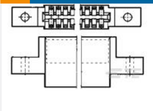
TE Part #2-583718-7 TW-LEAF CRP HSG 32 POS 100C/L
